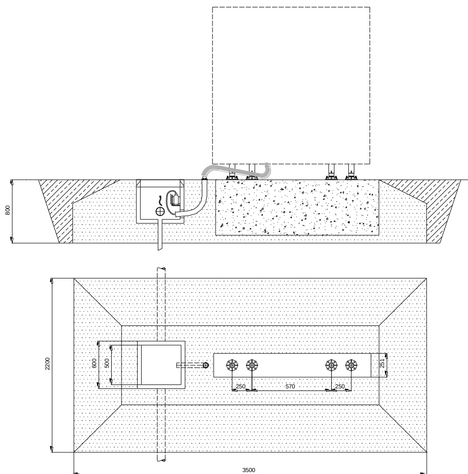
Figure 4 – Concrete foundation
