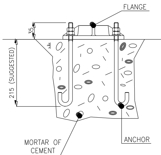
Figure 3 – Flange installation with anchor bolts
