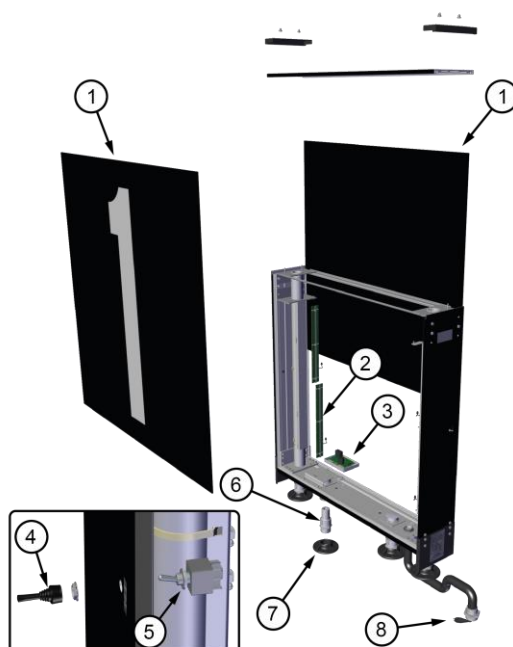
Figure 5 – Exploded view
