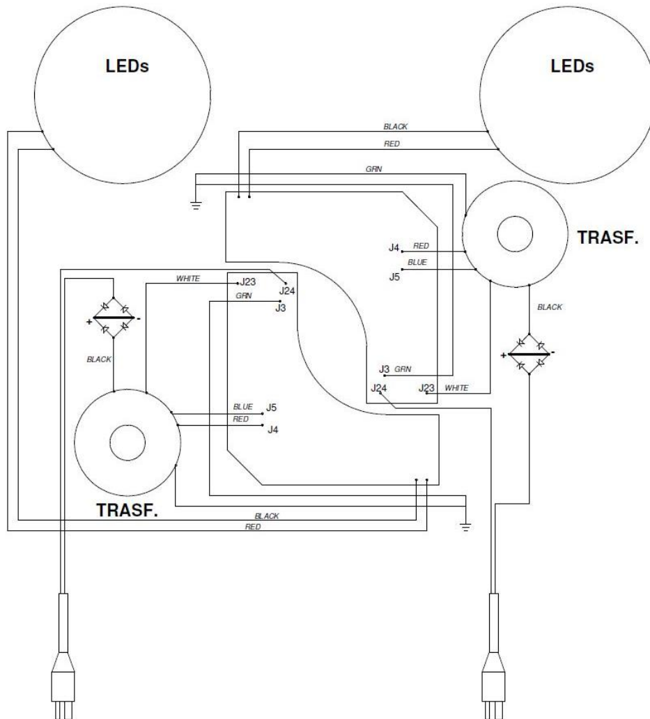
Figure 16 - Non-monitored series circuit power supply with external synchronization
