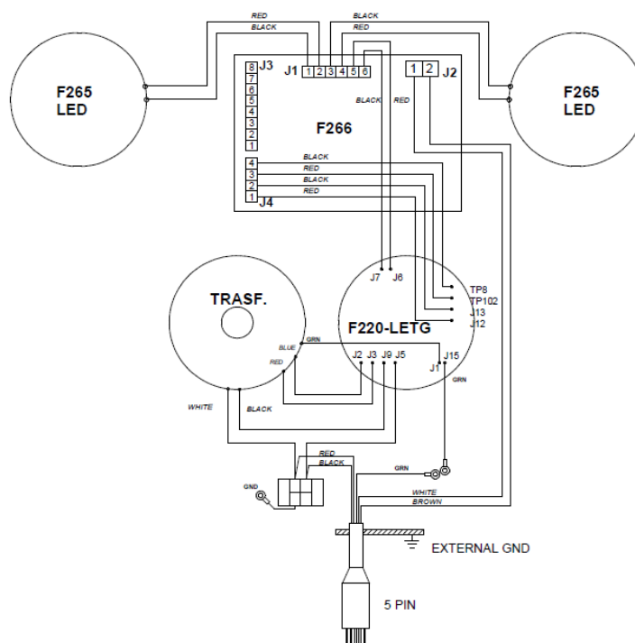
Figure 10– Monitored series circuit power supply
