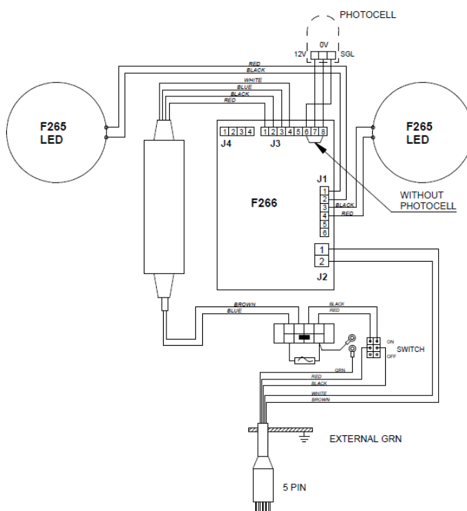
Figure 15– Monitored parallel circuit power supply with switch, with or without photocell
