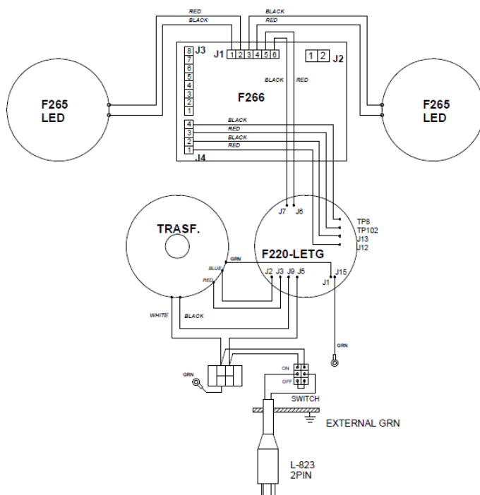
Figure 9– Non-monitored series circuit power supply with switch
