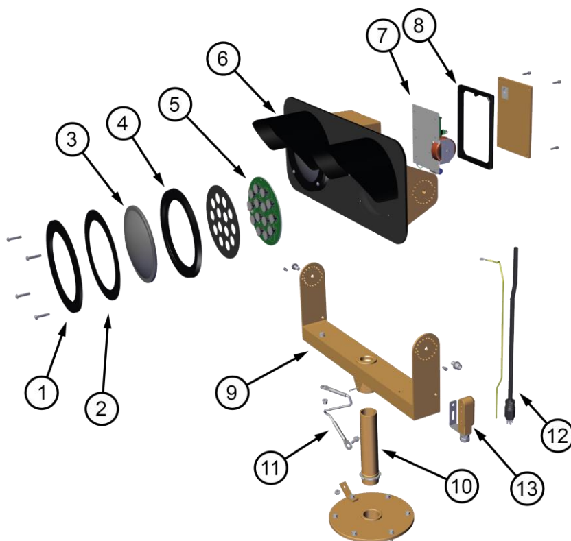
Figure 18 – Exploded View
