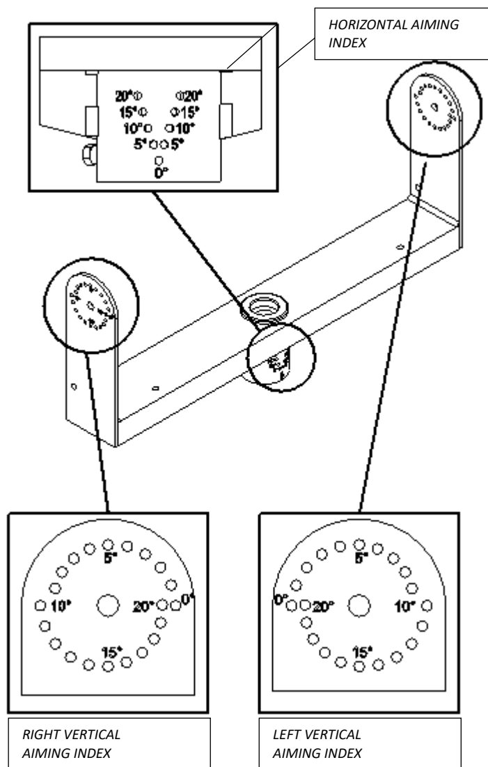
Figure 5 - Horizontal and vertical aiming indexes
