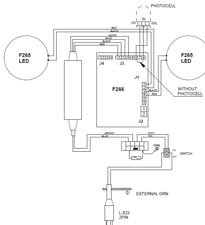
Figure 13– Non-monitored parallel circuit power supply with switch, with or without photocell
