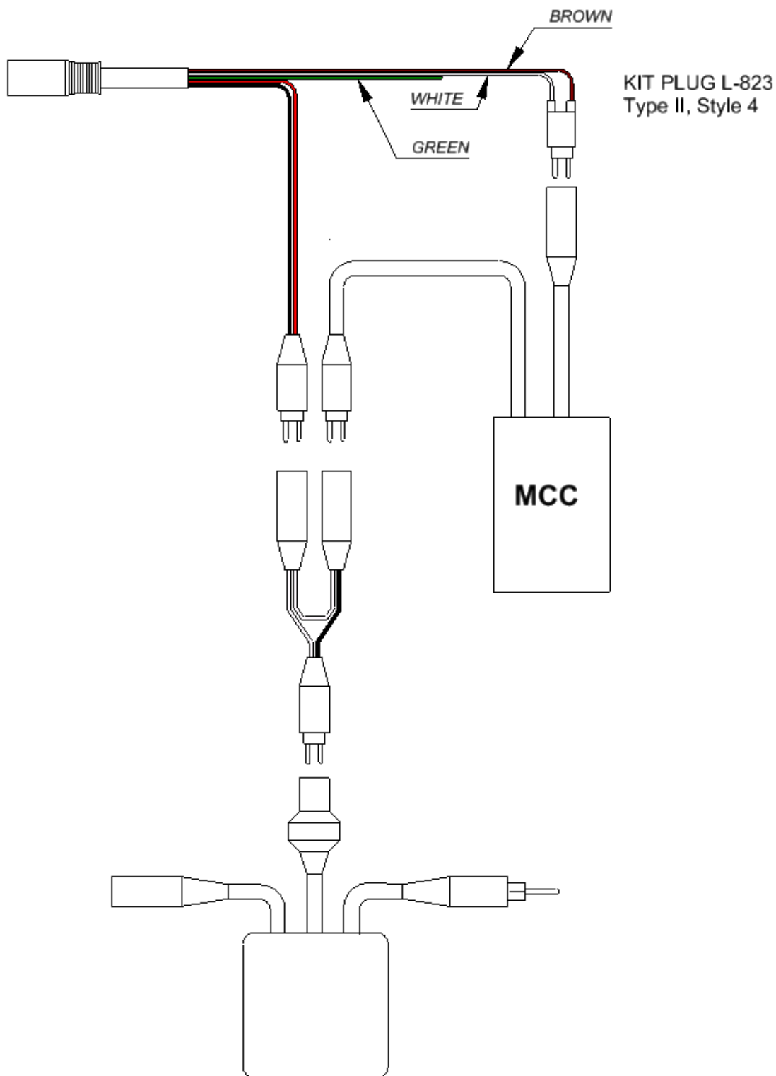
Figure 17 – Wiring diagram for connection of monitored LETG to transformer.
