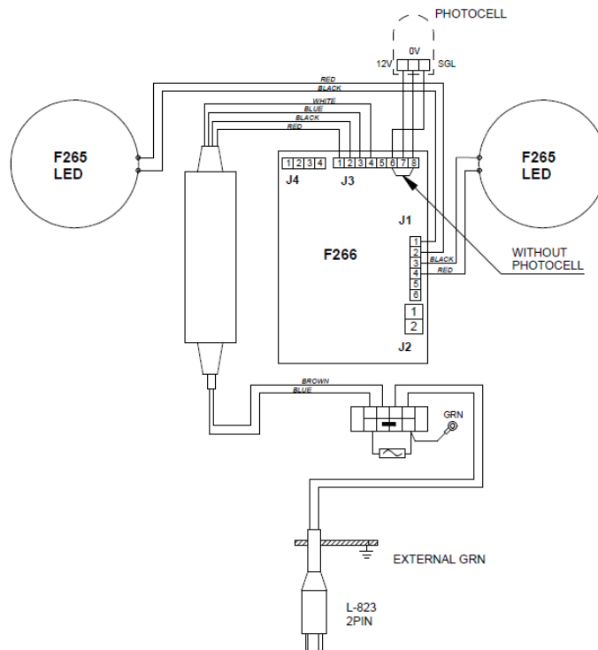
Figure 12– Non-monitored parallel circuit power supply with or without photocell
