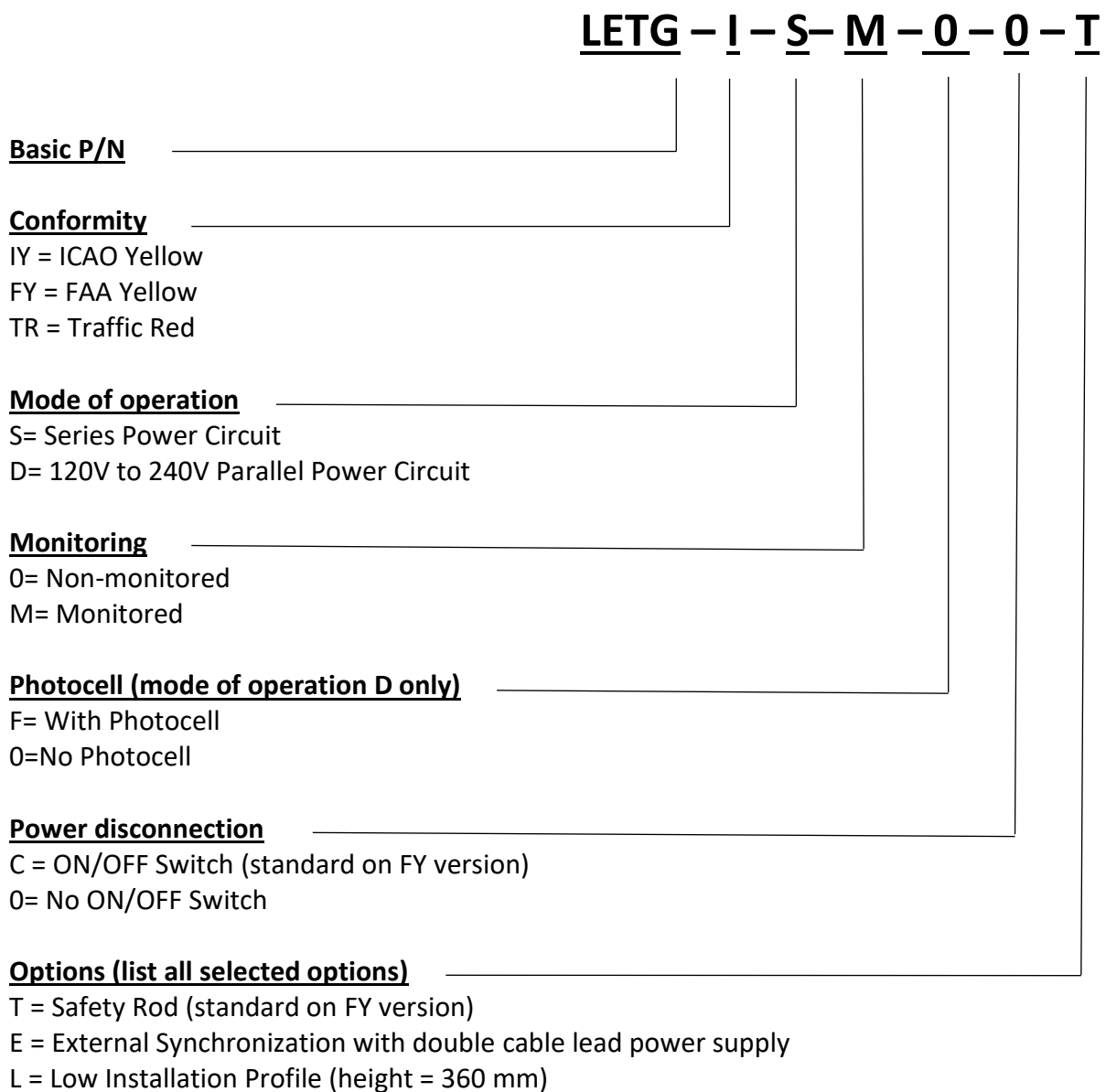
Figure 2 - P/N explanation
