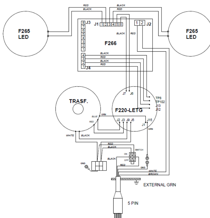
Figure 11– Monitored series circuit power supply with switch
