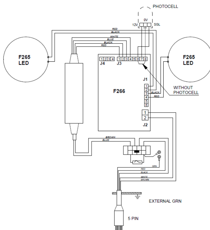
Figure 14– Monitored parallel circuit power supply with or without photocell
