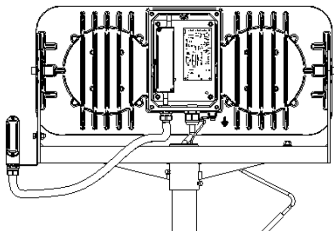
Figure 7 - Housing of parallel power supply unit with dusk sensor
