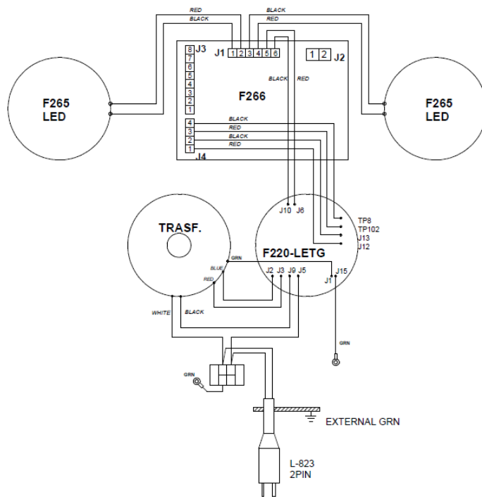
Figure 8– Non-monitored series circuit power supply
