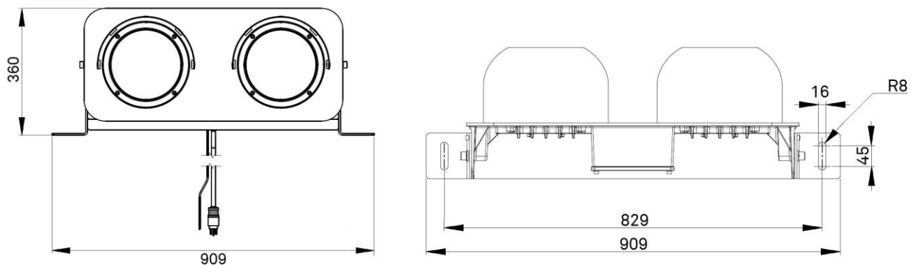
Figure 4 – LETG installation in low installation profile.
