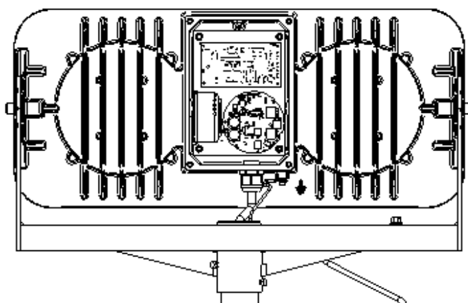
Figure 6 - Series power supply unit housing
