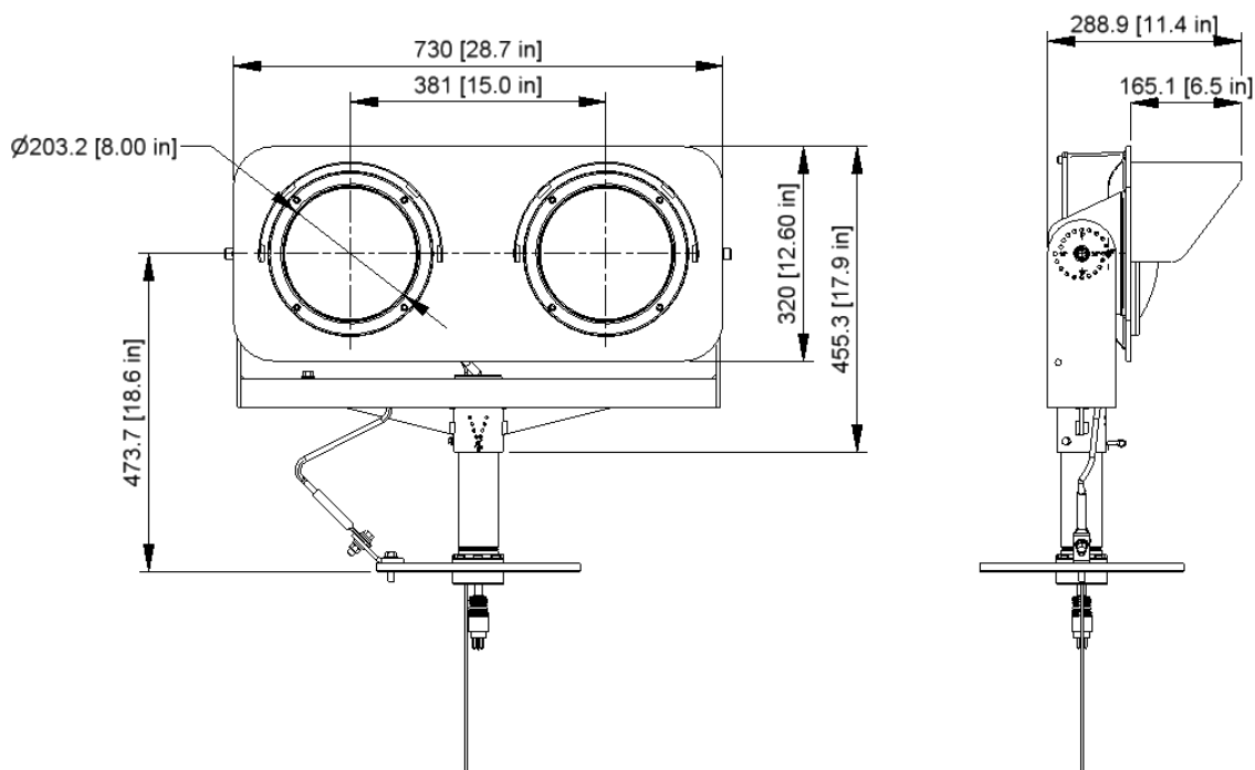
Figure 1 - Overall dimensions
