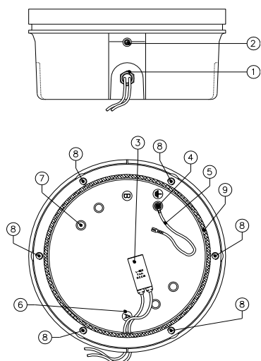
Figura 8 – Base Bassa Standard 12"
