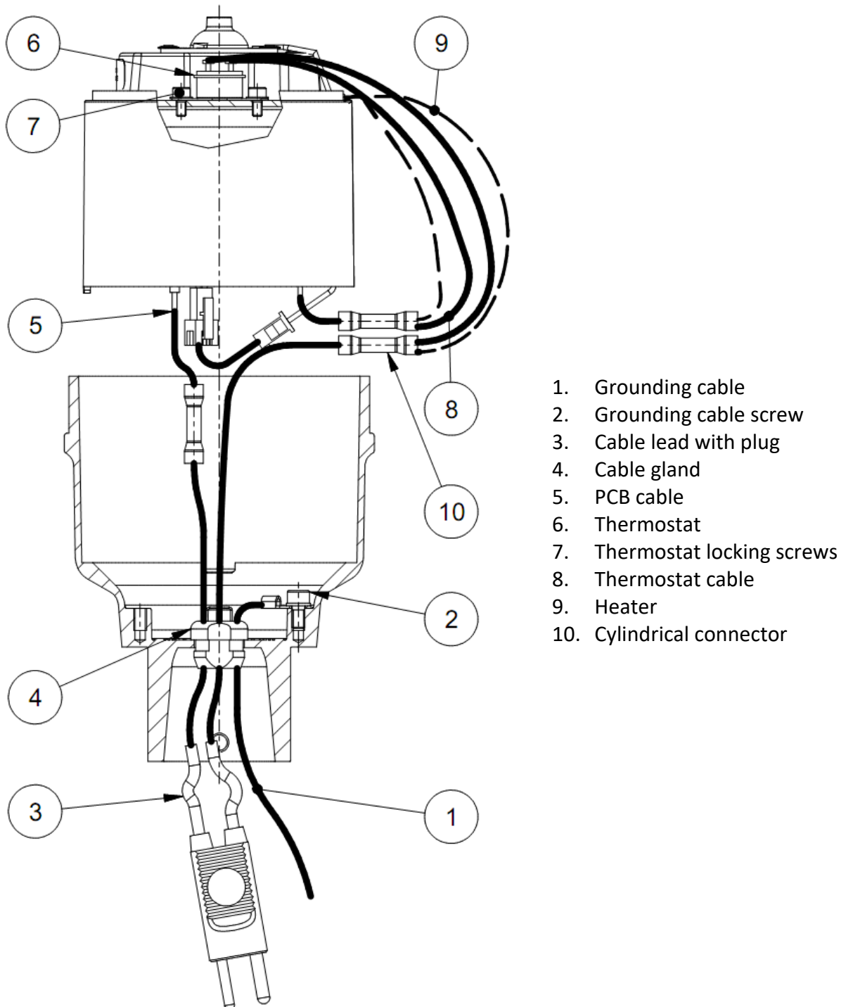
Figure 8 – Cable lead with plug, Grounding cable and Arctic kit
