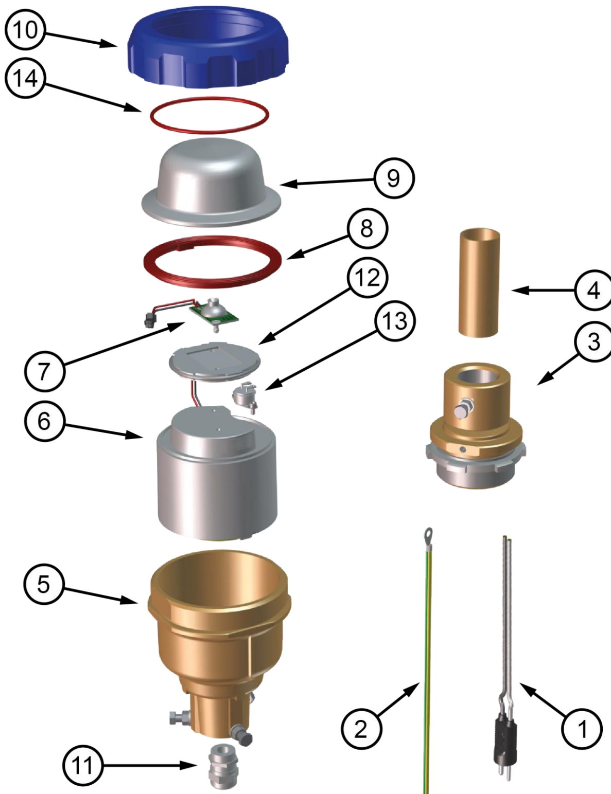
Figure 1 – Exploded View
