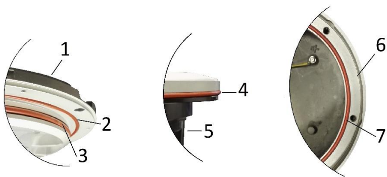
Figure 18 – Fixture Gaskets
