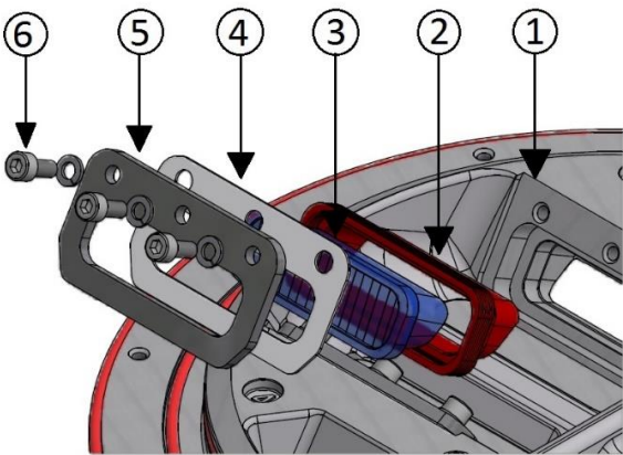
Figure 24 – Prism Gasket
