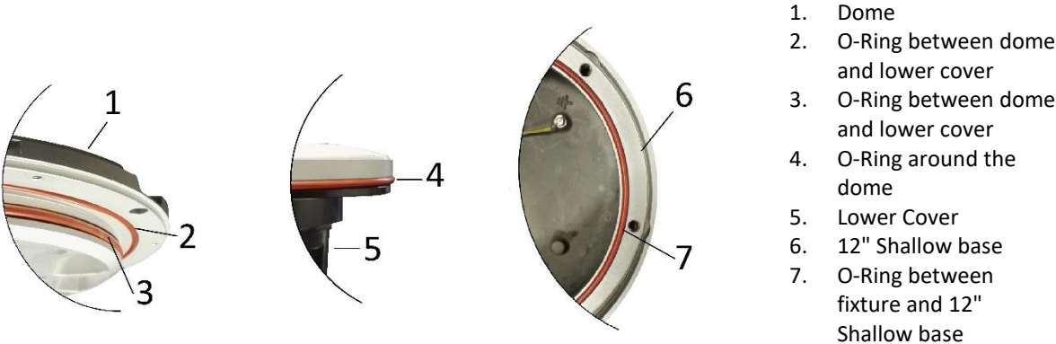
Figure 23– Fixture Gaskets
