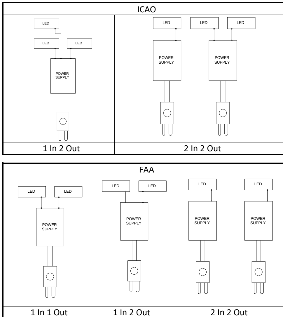
Figure 4 – Wiring Diagram
