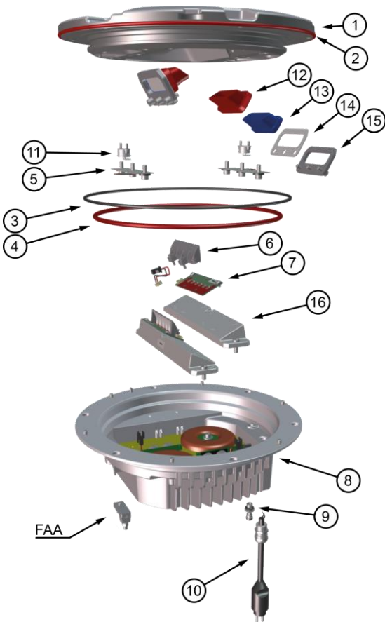
Figure 5 – Exploded View
