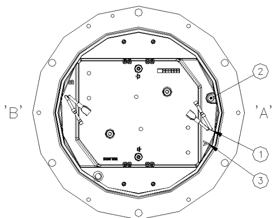
Figure 3 – Lower Cover Inside View
