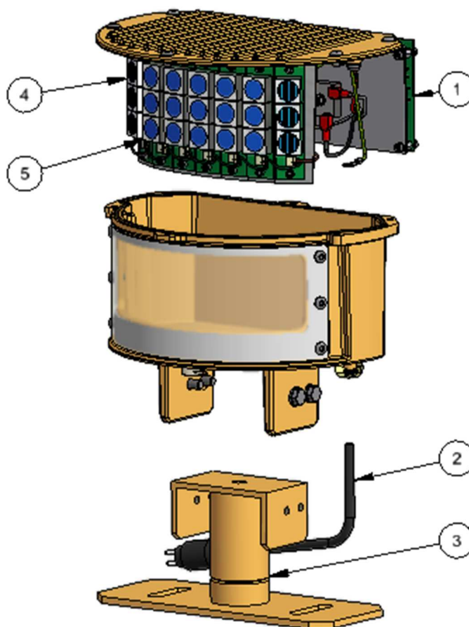
Figure 1 - Exploded view
