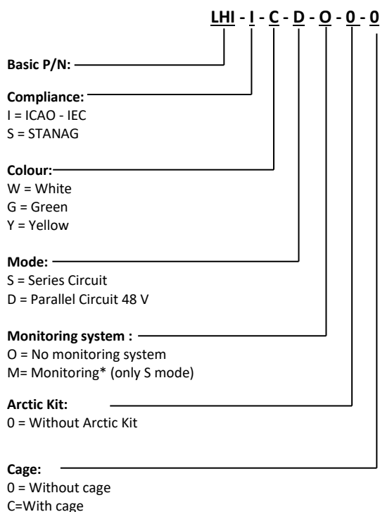
Figure 7 - Complete P/N identification
