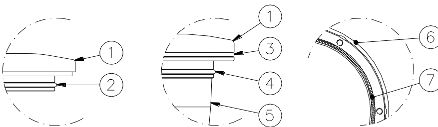
Figure 24– Fixture Gaskets
