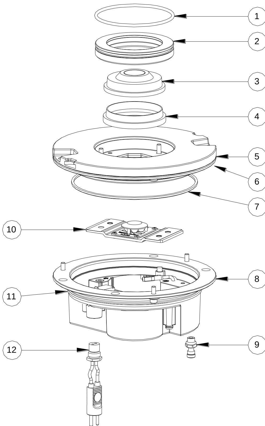
Figure 5 – Exploded View
