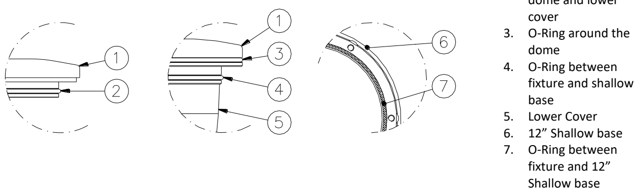
Figure 20 – Fixture Gaskets
