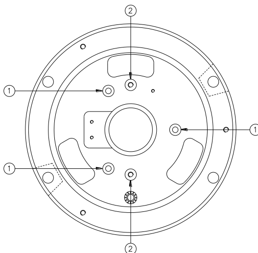
Figure 17 – Removing the Aluminium Ring
