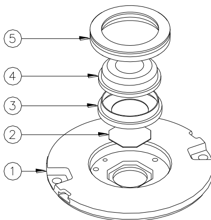
Figure 28 – Lens Gasket
