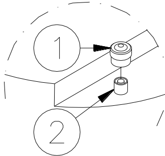
Figure 21 - Lower Cover with Pressure Valve
