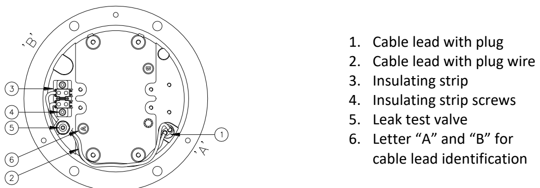
Figure 3 – Lower Cover Inside View
