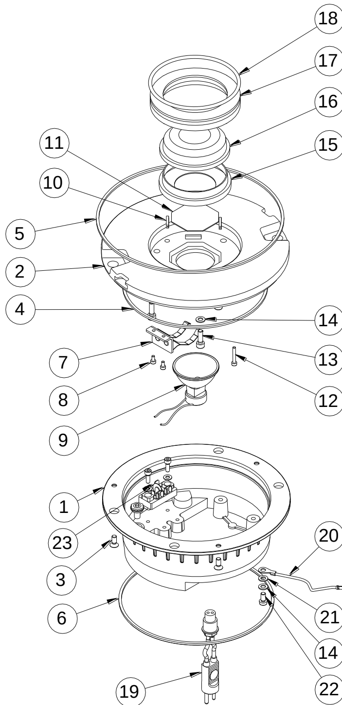
Figure 5 – Exploded View
