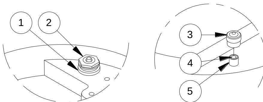
Figure 31 - Lower Cover with Pressure Valve
