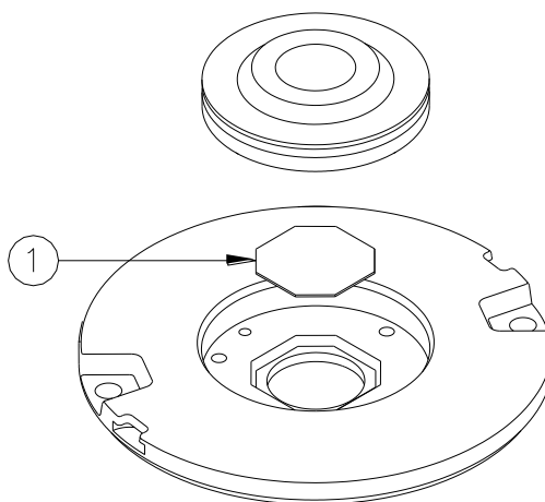
Figure 25 - Filter Replacement
