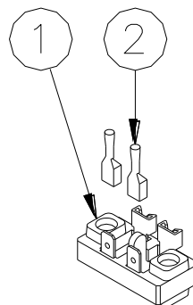
Figure 29 - Insulating Strip Female Faston
