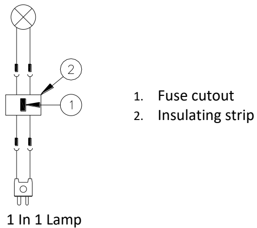
Figure 4 – Wiring Diagram
