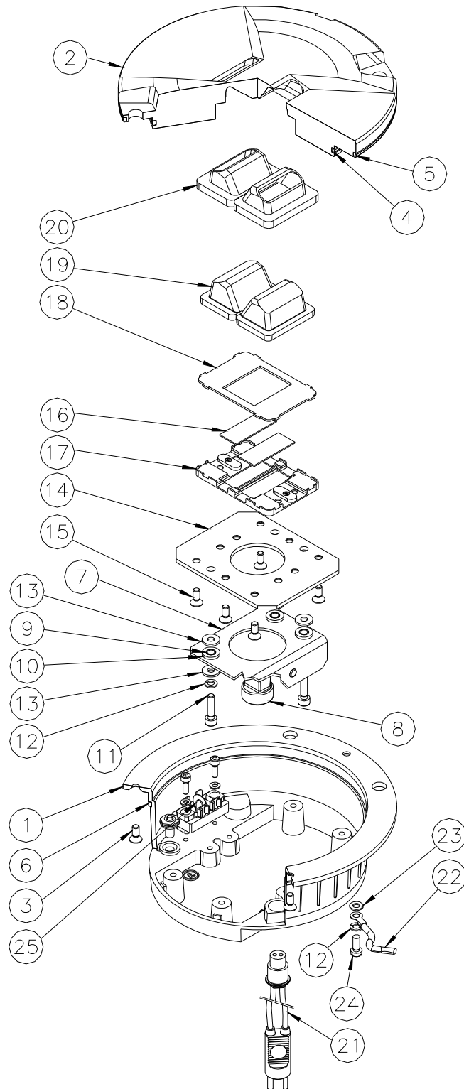
Figure 5 – Exploded View
