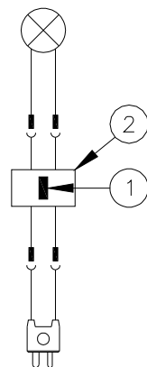
Figure 4 – Wiring Diagram
