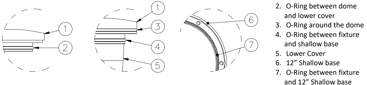
Figure 30– Fixture Gaskets
