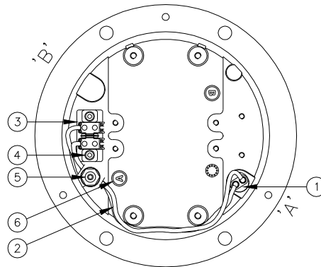
Figure 3 – Lower Cover Inside View
