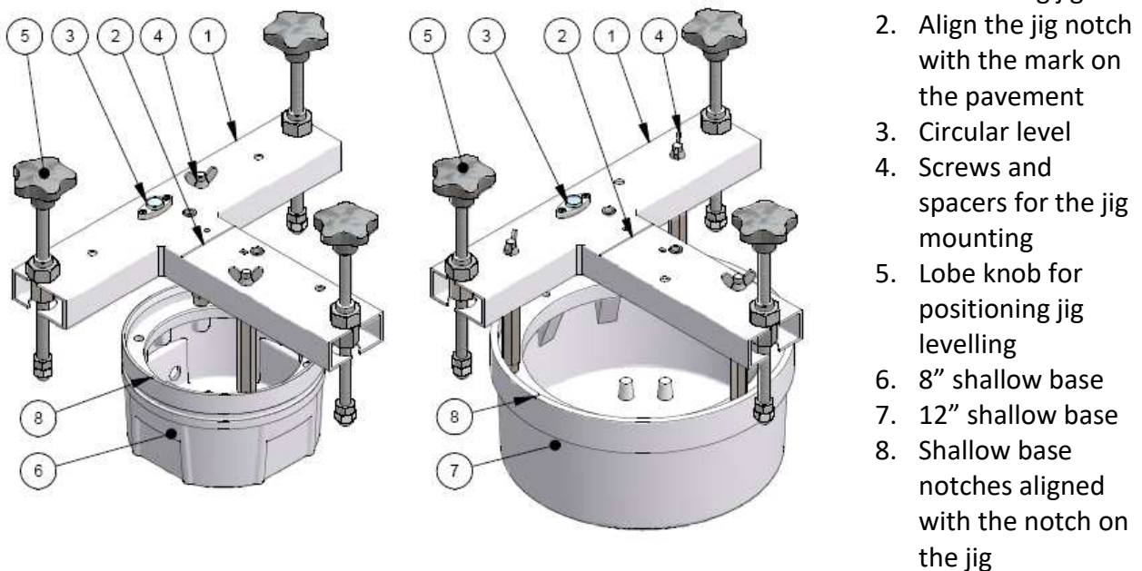
Figure 18 – Shallow base installation details
