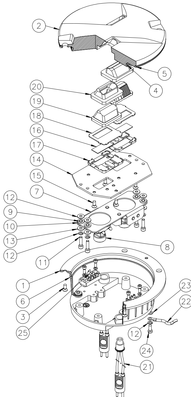
Figure 5 – Exploded View
