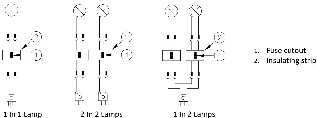
Figure 4 – Wiring Diagram
