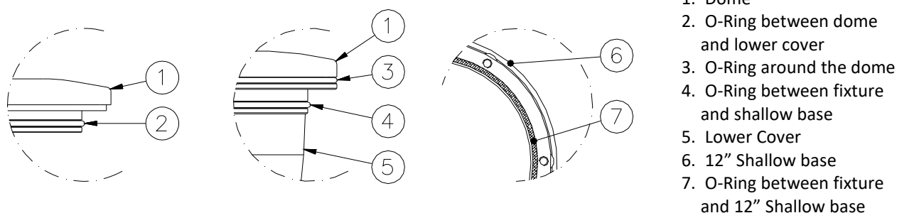
Figure 25 – Fixture Gaskets
