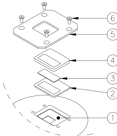
Figure 28 - Filter Replacement
