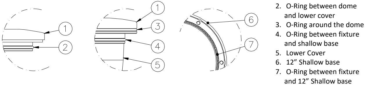
Figure 30– Fixture Gaskets
