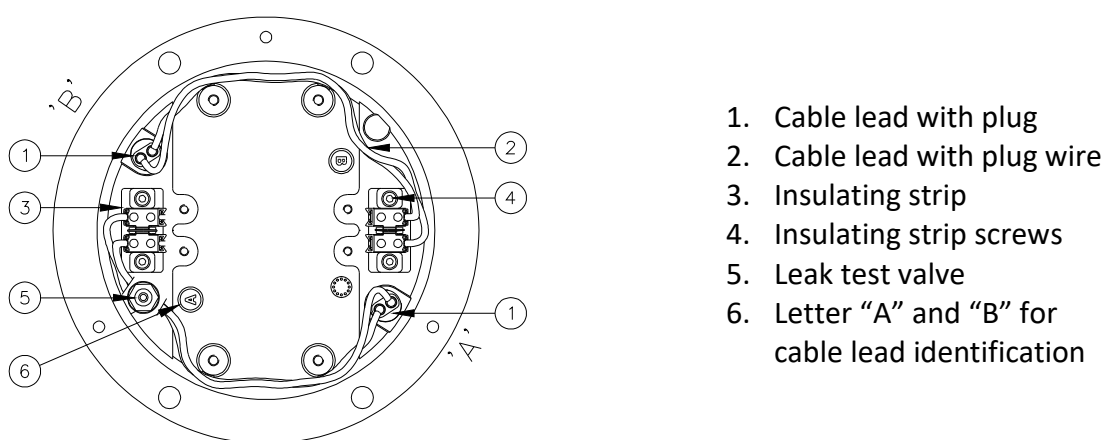
Figure 3 – Lower Cover Inside View
