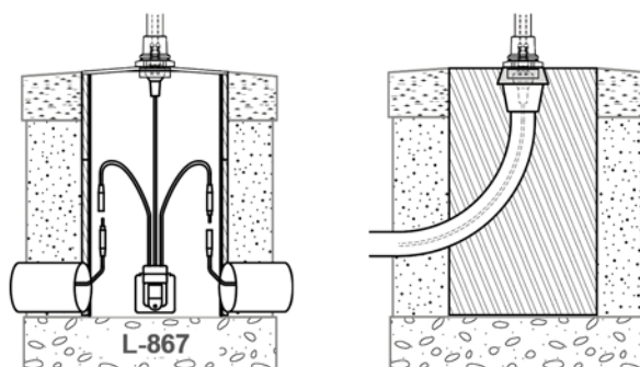
INSTALLATION EXAMPLE
