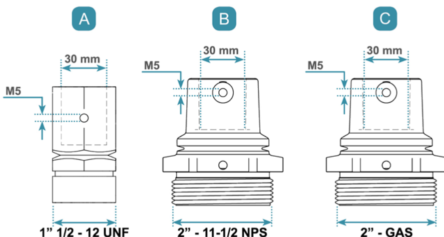
INSTALLATION EXAMPLE
