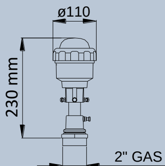
Overall Dimensions
