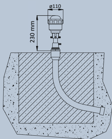
Pipe Elbow
