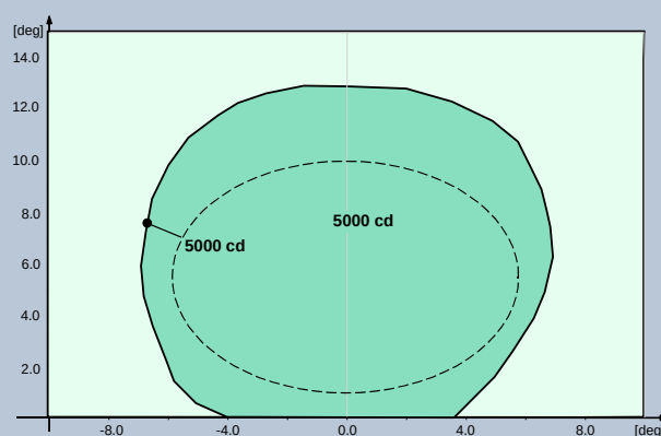
Fig. 2 Umbral FAA L-850E – Verde
