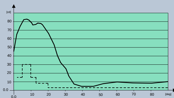
Fig. 2 ICAO fig. 5.9 Illustration 6 TLOF – Green
