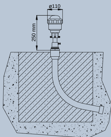
Pipe Elbow
