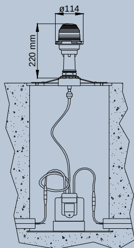
FAA L-867 Deep Base and Base Plate
