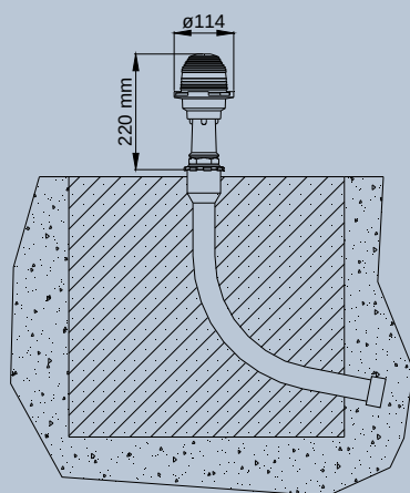
Pipe Elbow
