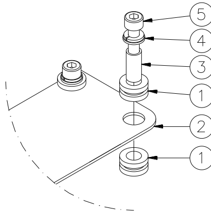
Figure 30 - Vibration-Damping Block
