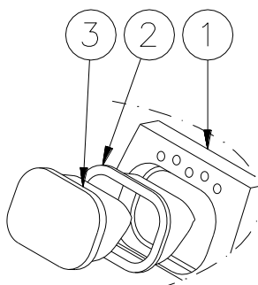
Figure 27 – Prism Gasket
