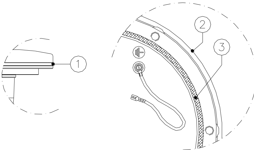
Figure 13 – Gaskets for 12" shallow base
