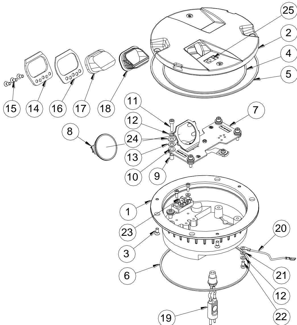
Figure 5 – Exploded View
