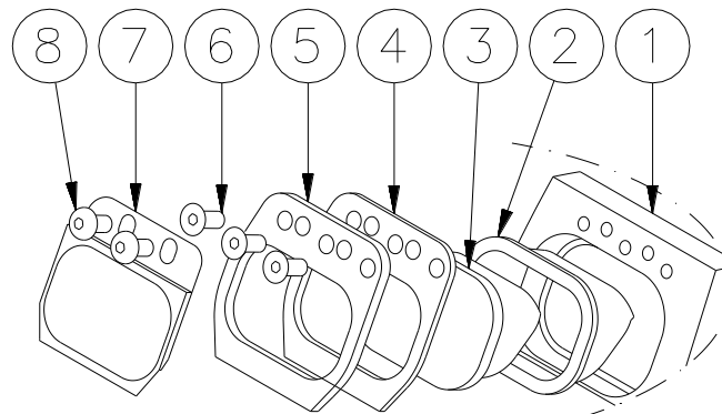
Figure 24 - Prism Replacement
