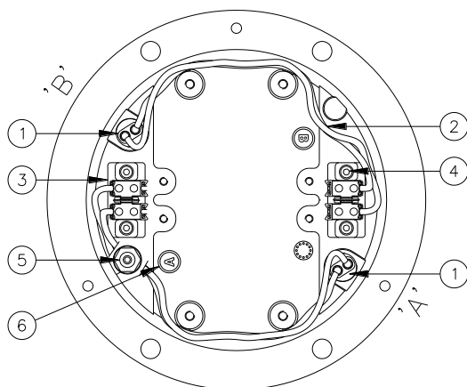
Figure 3 – Lower Cover Inside View
