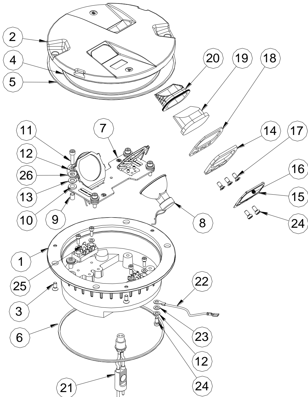
Figure 5 – Exploded View
