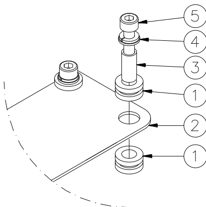
Figure 31 - Vibration-Damping Block
