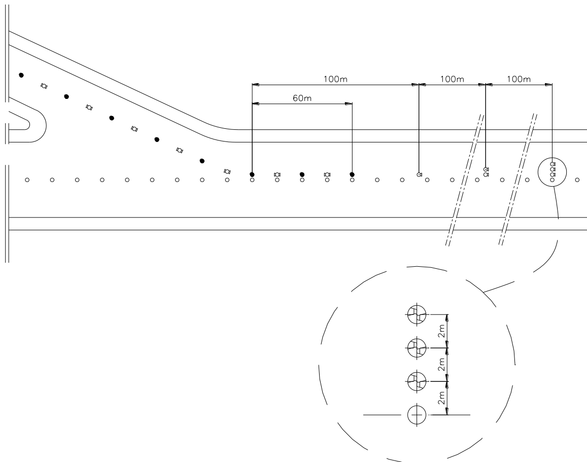
Figure 12 – R.E.T.I.L. Configuration
