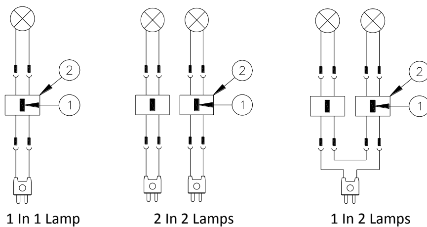
Figure 4 – Wiring Diagram
