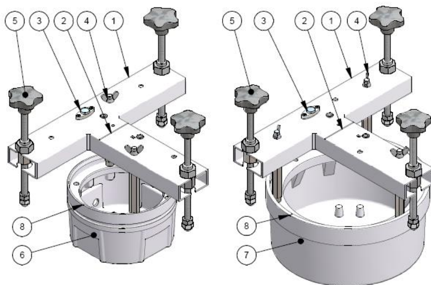
Figure 17 – Shallow base installation details
