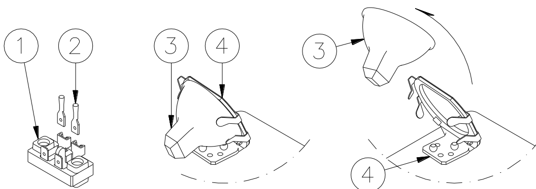
Figure 26 - Relamping
