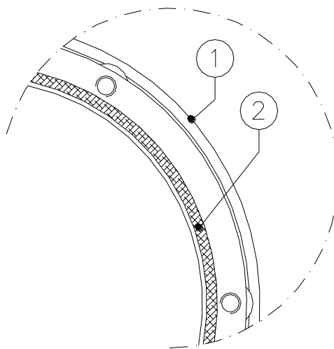
Figure 19 – Gaskets for L-868 base
