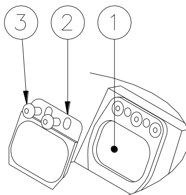
Figure 23 - Prism Cleaning
