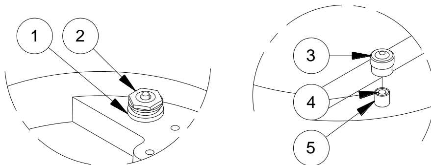
Figure 32 - Lower Cover with Pressure Valve
