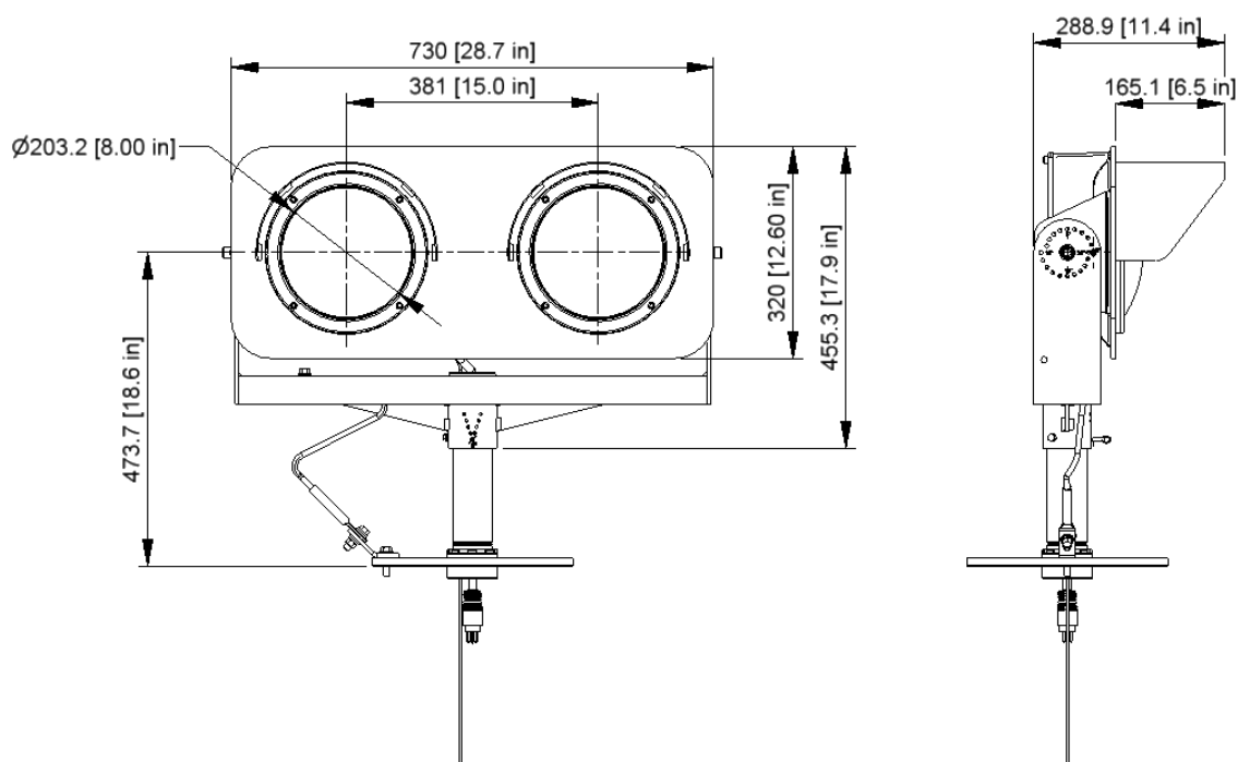
Figure 1 - Overall dimensions
