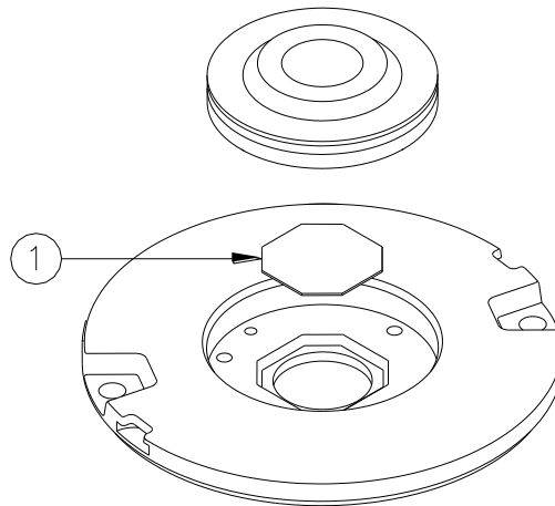
Figure 24 - Filter Replacement
